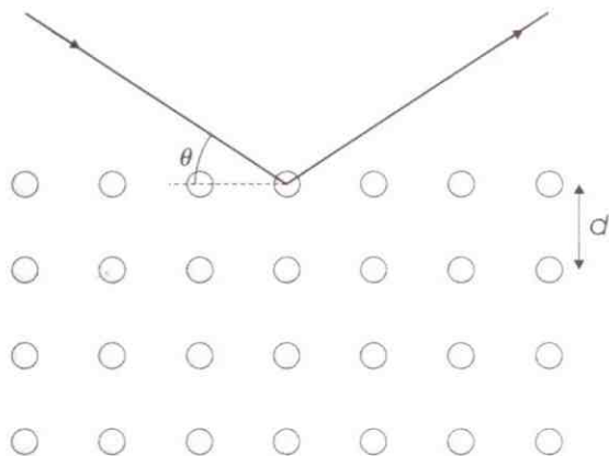
Figure 2.34 Electron waves are diffracted by planes of atoms separated by the interplanar spacing d when the Bragg equation ( n\lambda = 2d \sin \theta ) is obeyed
