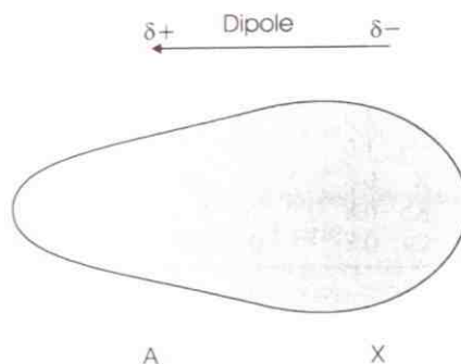
Figure 2.11 The electron density in a bonding molecular orbital between two dissimilar atoms is distorted so that the end nearer to the nonmetallic atom attracts more of the charge cloud. The bond is then an electric dipole, with charges \delta+ and \delta- , represented by an arrow pointing from the negative to the positive charge
