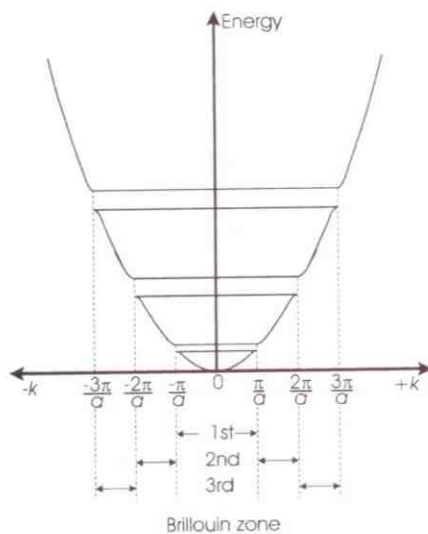
Figure 2.37 The first three Brillouin zones for a one-dimensional crystal with atom spacing a
