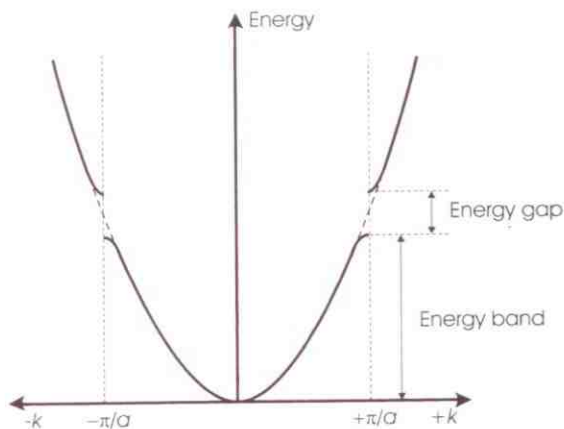
Figure 2.33 The one-dimensional free-electron curve of energy, E , versus wavenumber k ; it is 'broken up' into energy bands separated by energy gaps because of the periodic potential of atomic nuclei of separation a
