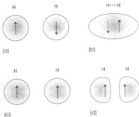
Figure 2.4 Isolated hydrogen atoms have spherically symmetrical 1s orbitals, each containing one s electron, represented as an arrow. Two atoms can have electrons in (a) an antiparallel or (c) parallel arrangement; (b), if the electrons have antiparallel spins the electron density accumulates between the nuclei to form a covalent bond; (d) if the electrons have parallel spins the electron density is low between the nuclei and no bond forms
