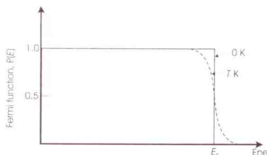
Figure 2.31 The Fermi function, P(E) , giving the probability of the occupation of an energy level as a function of the energy, E . At 0 K, the probability is 1.0 up to Fermi energy, E_F , and thereafter is 0. At higher temperatures, the curve changes smoothly from 1.0 to 0.
