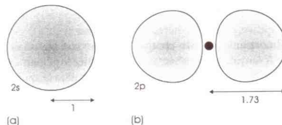
Figure 2.12 The relative extension of (a) a 2s orbital (1.0) and (b) a 2p orbital ( \sqrt{3} , 1.73)
