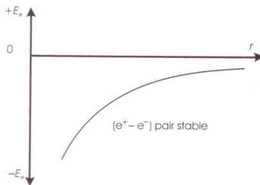
Figure 2.1 The attractive potential energy between a pair of monovalent ions, E_e , as a function of interionic separation, r . The energy is set at zero for ions that are at infinite separation
