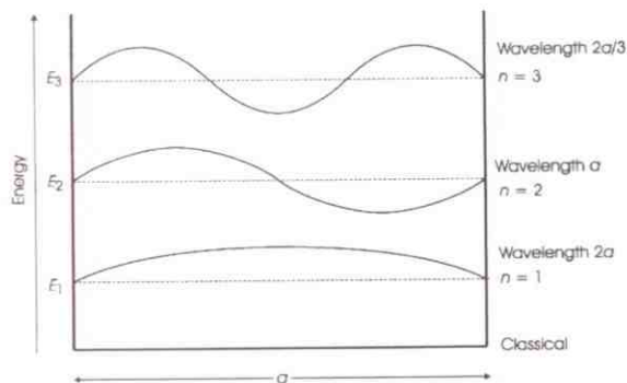
Figure 2.27 The energy levels of an electron confined to a line of length a . Quantum mechanics restricts the electron wave to fit into the length of the line, thus limiting the energy of the electron to discrete values corresponding to n = 1, 2, 3 and so on
