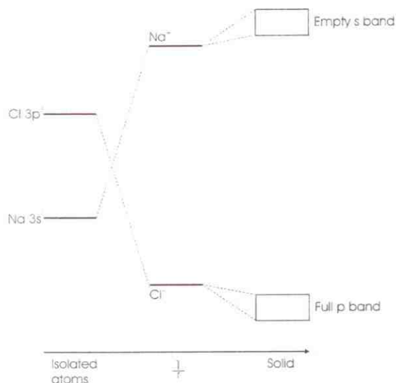
Figure 2.38 Energy bands of isolated atoms in sodium chloride (NaCl). As the spacing between the atoms, r , decreases, first ionisation occurs and then energy bands develop. These are narrow and widely separated, as expected from the ionic model of bonding
