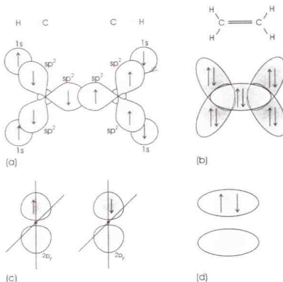
Figure 2.21 Bonding in ethene (ethylene), C_2H_4 . Overlap of the 1s orbitals of H with the sp^2 hybrid orbitals on C (part a) results in a \sigma bonded molecule (part b). Overlap of the 2p_z orbitals on C (part c), results in the formation of a \pi bonds (part d). The conventional representation of the double bond as C=C , does not convey the information that there are two different bond types
