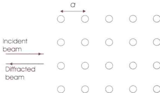
Figure 2.35 An electron wave normal to planes of atoms of interplanar spacing a will be diffracted back on itself when the wavelength \lambda is equal to 2na and the wave vector k is equal to 2n\pi/a
