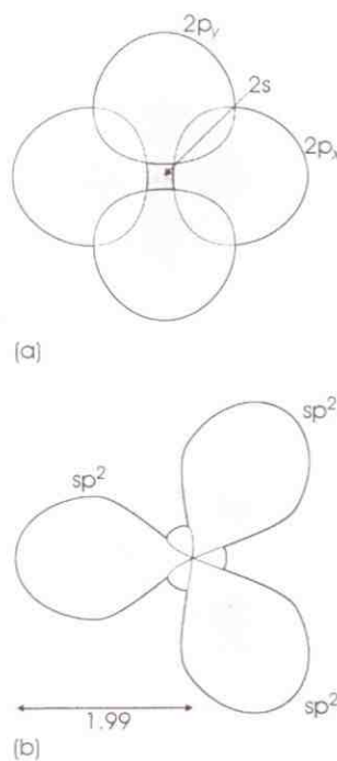
Figure 2.15 (a) The 2s, 2p x and 2p y orbitals on an atom and (b) the three sp^2 hybrid orbitals formed by combining the three original orbitals. Each hybrid orbital has a large lobe and a small lobe. The extension of the large lobe is 1.99, compared with 1.0 for a 2s orbital and 1.73 for a 2p x orbital. The orbitals are arranged at an angle of 120^\circ to each other and point towards the vertices of an equilateral triangle
