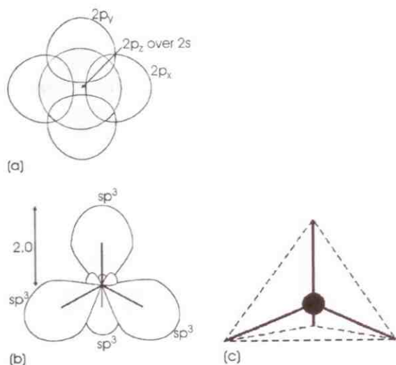
Figure 2.16 (a) The 2s , 2p_x , 2p_y and 2p_z orbitals on an atom; (b) the four sp^3 hybrid orbitals formed by combining the four original orbitals. Each hybrid orbital has a large lobe and a small lobe. The extension of the large lobe is 2.0, compared with 1.0 for a 2s orbital and 1.73 for a 2p_x orbital. (c) The orbitals are at an angle of 109.5^\circ to each other and point towards the vertices of a tetrahedron
