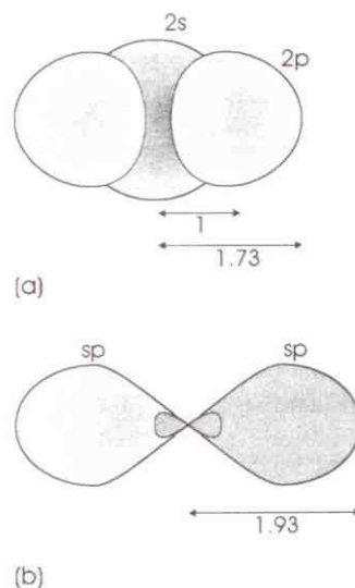
Figure 2.14 (a) The 2s and 2p_x orbitals on an atom and (b) the two sp hybrid orbitals formed by combining the 2s and 2p_x orbitals. Each hybrid orbital has a large lobe and a small lobe. The extension of the large lobe is 1.93, compared with 1.0 for a 2s orbital and 1.73 for a 2p_x orbital. The orbitals point directly away from each other
