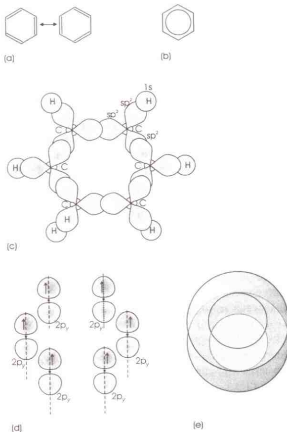
Figure 2.22 Bonding in benzene, C_6H_6 . (a) Conventional bonding diagrams for the two main alternative resonance hybrid structures of the benzene molecule. The lines indicate bonds between carbon atoms, which lie at the vertices of a hexagon. Each carbon is linked to one hydrogen atom (omitted) and two carbon atoms. (b) The benzene molecule is often drawn as a hexagon enclosing a circle, to indicate the resonance nature of the bonding. The bonding is more complicated than the conventional diagrams indicate. Overlap of the 1s orbitals of H with the sp^2 hybrid orbitals on C (part c) results in a \sigma bonded hexagonal molecule. Overlap of the 2p_y orbitals on C (part d), results in the formation of \pi bonds (part e). The lobes of the \pi bonds lie above and below the plane of the C-H planar structure, and delocalisation means that the orbitals are spread equally over the ring. The representation of the molecule in part (b) attempts to convey some of this information
